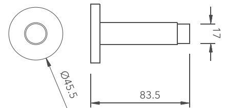
SCLDS006SS Mounted on door or on wall Material: Stainless steel
