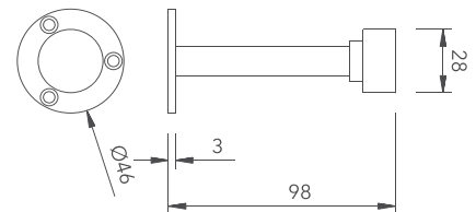
SCLDS004SS Mounted on door or on wall Material: Stainless steel
